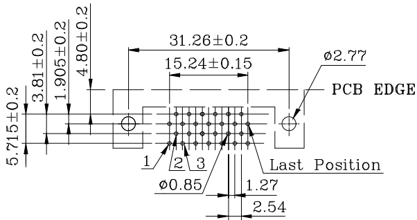
PCB Layout (A)
