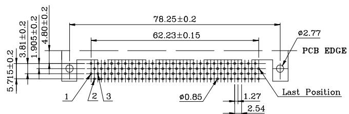
PCB Layout (B)
